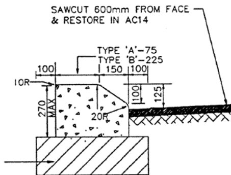
MOUNTABLE KERB
