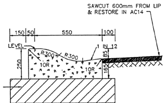
ROLL KERB
