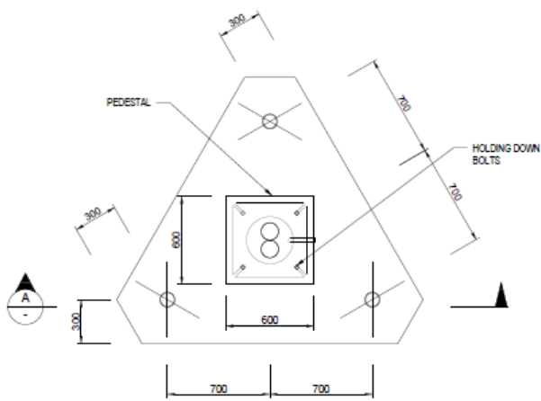
A25-20-100-89 - POLE PAD SCALE 1:20
